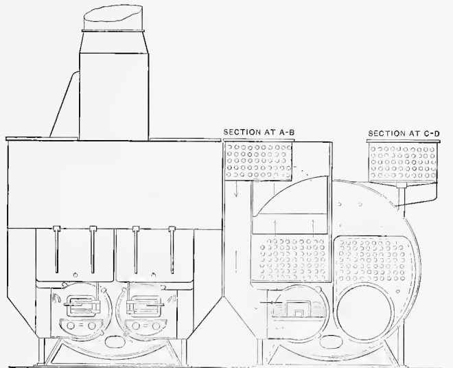
FIG. 1.—BOILER WITH COMMON TUBES.
